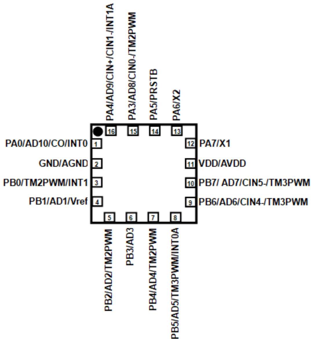
PMS171B-1J16A (QFN3*3-16P-0.5pitch)
