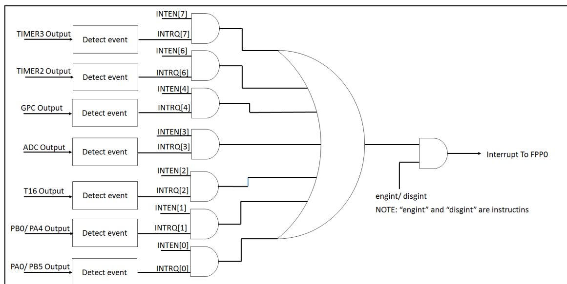
Fig. 16: Hardware diagram of interrupt controller
