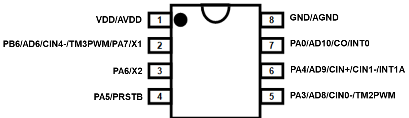
PMS171B-S08B (SOP8-150mil)
