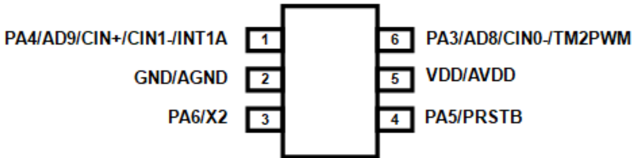
PMS171B-U06 (SOT23-6 60mil)
