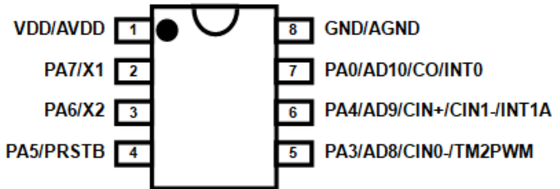
PMS171B-S08 (SOP8-150mil)
