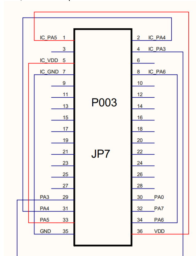
Fig.21: schematic diagram of PMS161-S08B Jumper7 when using p003
