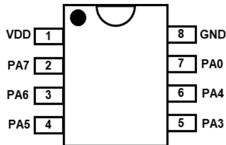
PMS15A/ PMS150C - S08: SOP8 (150mil) PMS15A/ PMS150C - D08: DIP8 (300mil)
