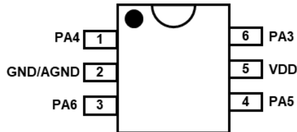
PMS15A/ PMS150C - U06: SOT23-6 (60mil)
