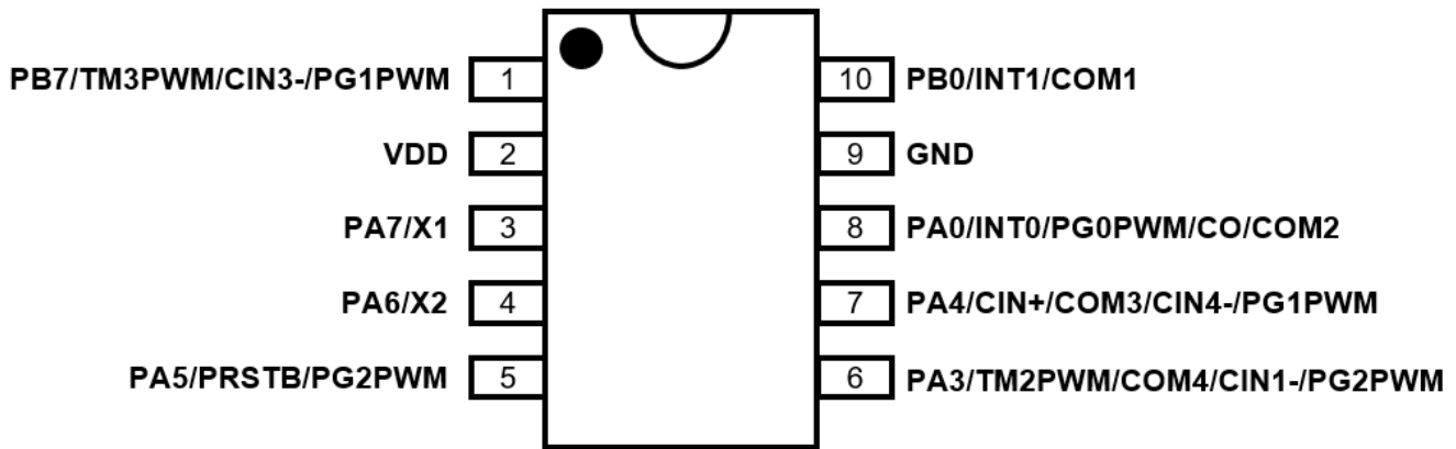
PMS154G-M10:MSOP10(118mil)
