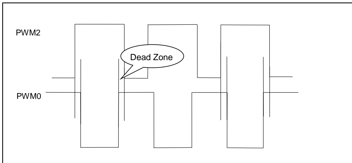
Fig.16: Complementary PWM waveform with dead zones
