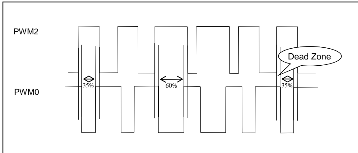
Fig.17: Complementary PWM waveform with dead zones
