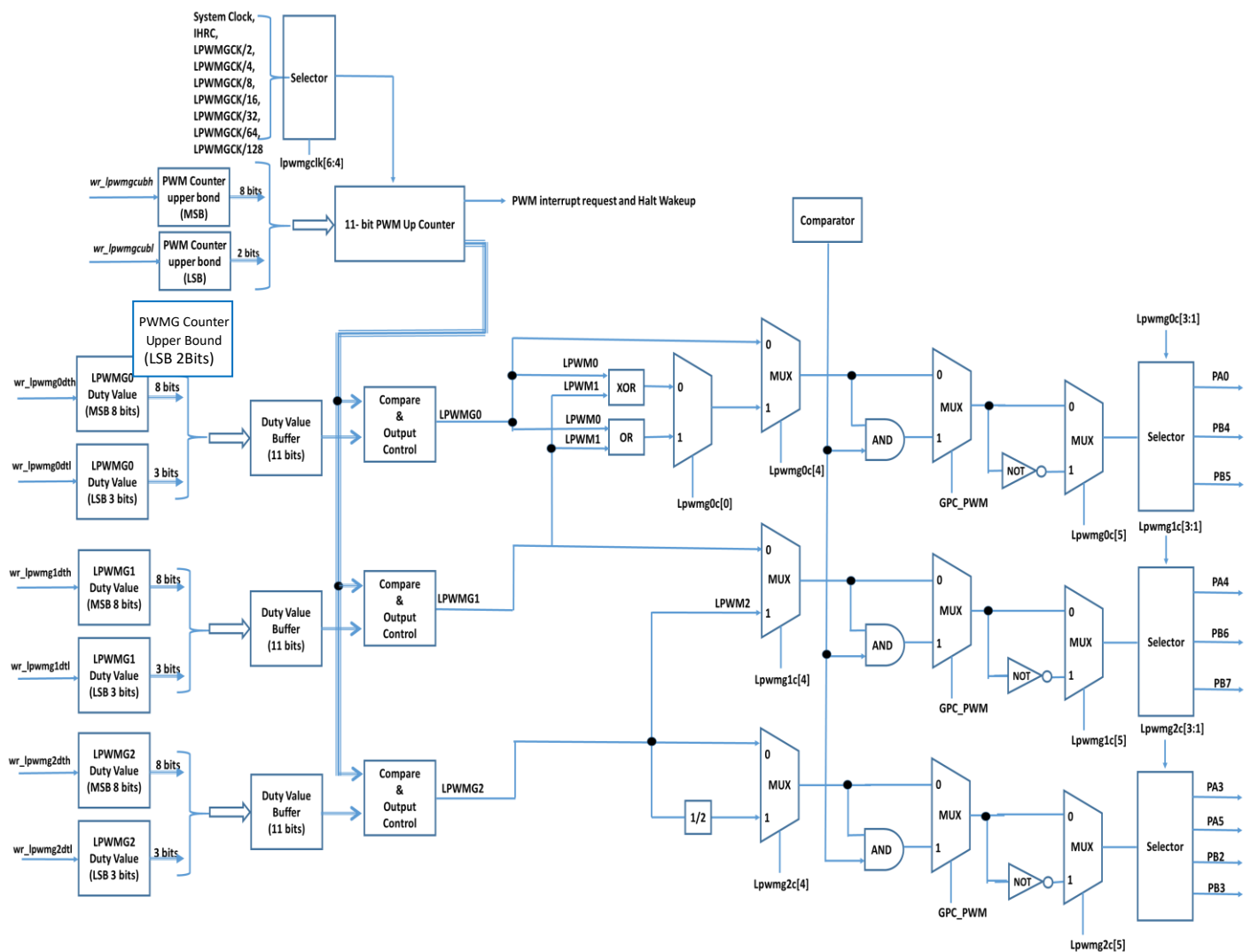
Fig.14: Hardware diagram of whole set of triple SuLED 11-bit PWM generators
