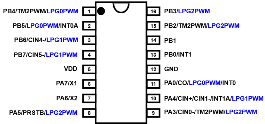
PMS152-S16 (SOP16-150mil)
